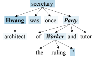
Figure 8: More examples and the pruned dependency trees the C-GCN predicted correctly. Words are shaded by the number of dimensions they contributed to h_{\text{sent}} in the pooling operation, with punctuation omitted.
