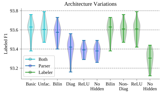
Figure 3: Performance of architecture variations: our basic+lemma system; unfactorized (labeler-only); with bilinear classifiers (Eq. 3); with non-diagonal tensors in the labeler or diagonal tensors in the parser; with the ReLU nonlinearity; omitting the hidden layers (Eqs. 5–8).
